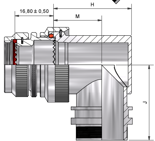
90° BACKSHELL - TYPE 2
