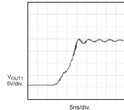
Output Rise-Time
