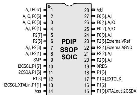
Figure 5. CY8C27443 28-Pin PSoC Device
