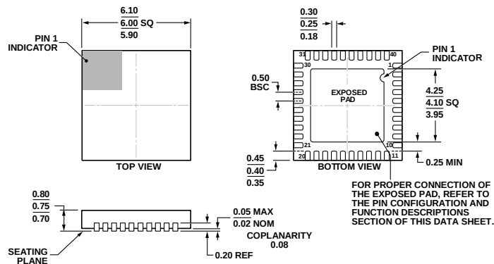
Figure 81. 40-Lead Lead Frame Chip Scale Package [LFCSP_WQ] 6 mm × 6 mm Body, Very, Very Thin Quad (CP-40-9)
