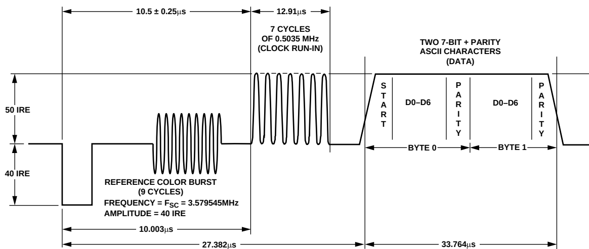
Figure 56. Closed Captioning Waveform (NTSC)
