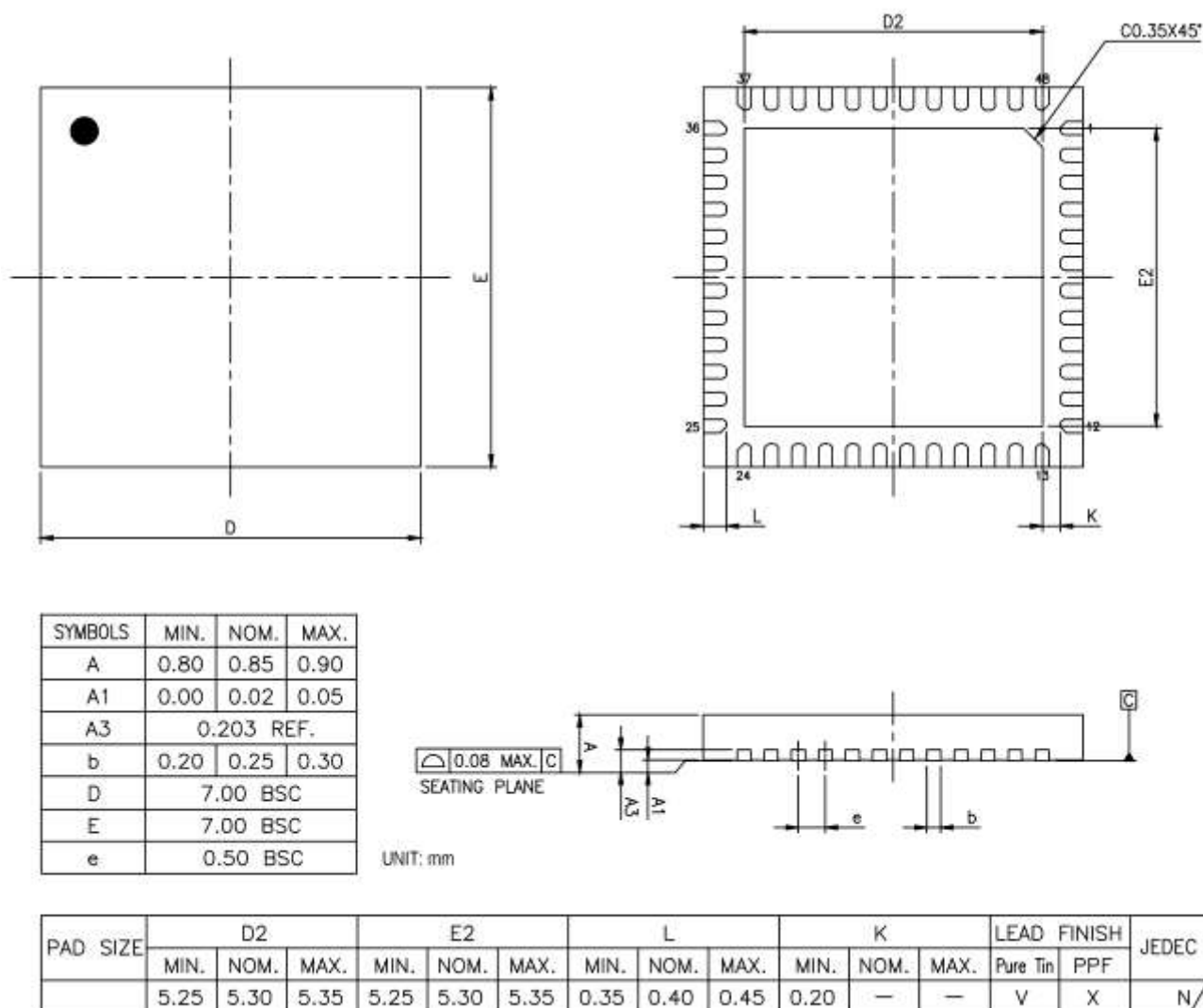
Figure 7-3 QFN-48 Package Dimensions
