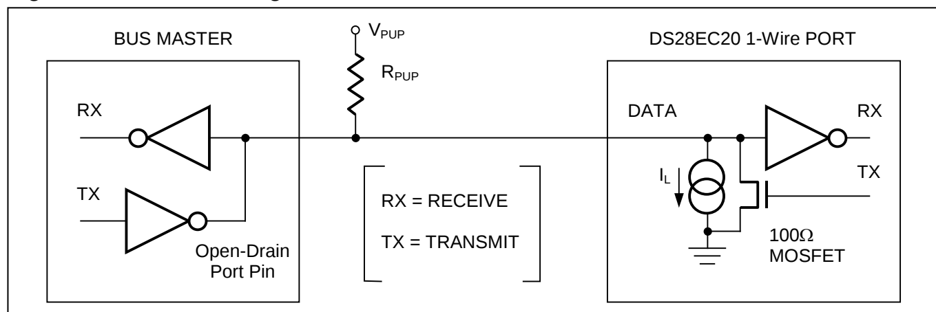
Figure 8. Hardware Configuration
