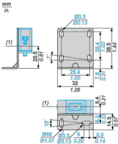
(1) Optical axis
