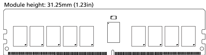
Figure 1: 288-Pin RDIMM (MO-309, R/C-C1, R/C-C2)
