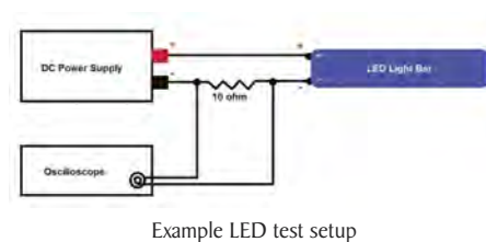
Example LED test setup
