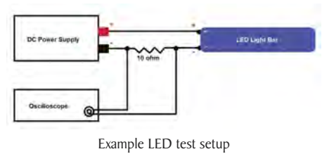
Example LED test setup
