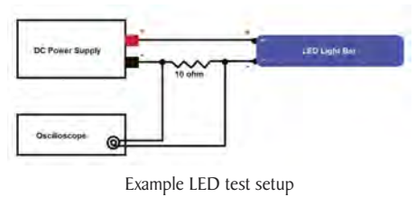
Example LED test setup
