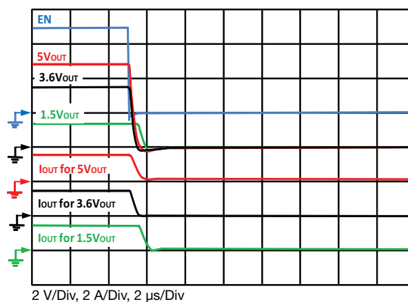
Figure 21 - Typical Fall Time C_{OUT} = 0.1 \mu F , C_{IN} = 4.7 \mu F , I_{OUT} = 1.5 A
