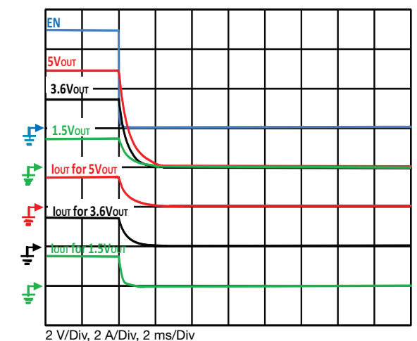
Figure 23 - Typical Fall Time C_{OUT} = 200 \mu F , C_{IN} = 4.7 \mu F , I_{OUT} = 1.5 A
