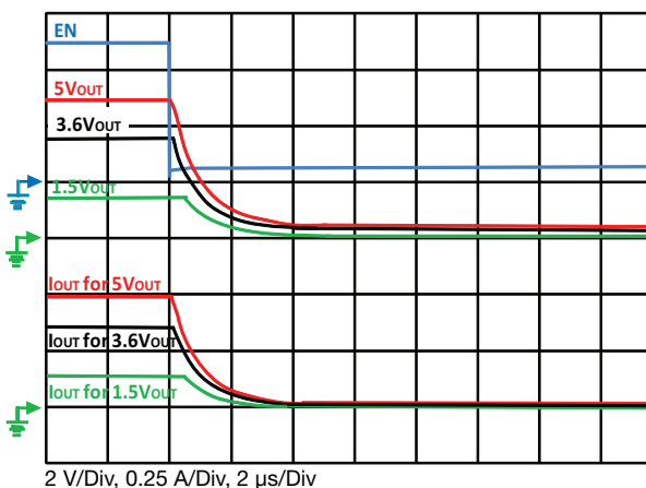
Figure 22 - Typical Fall Time C_{OUT} = 0.1 \mu F , C_{IN} = 4.7 \mu F , R_{OUT} = 10 \Omega
