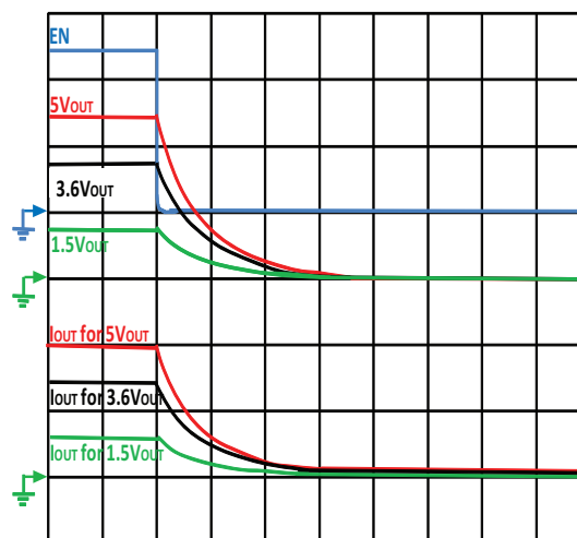
Figure 25 - Typical Fall Time
