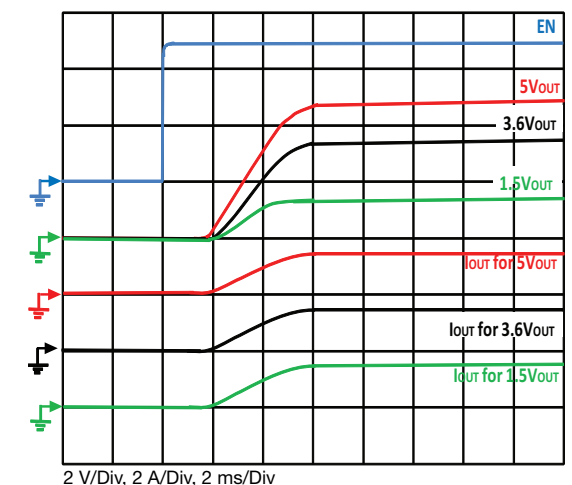
Figure 20 - Typical Turn-on Delay, Rise Time C_{OUT} = 200 \mu F , C_{IN} = 4.7 \mu F , I_{OUT} = 1.5 A
