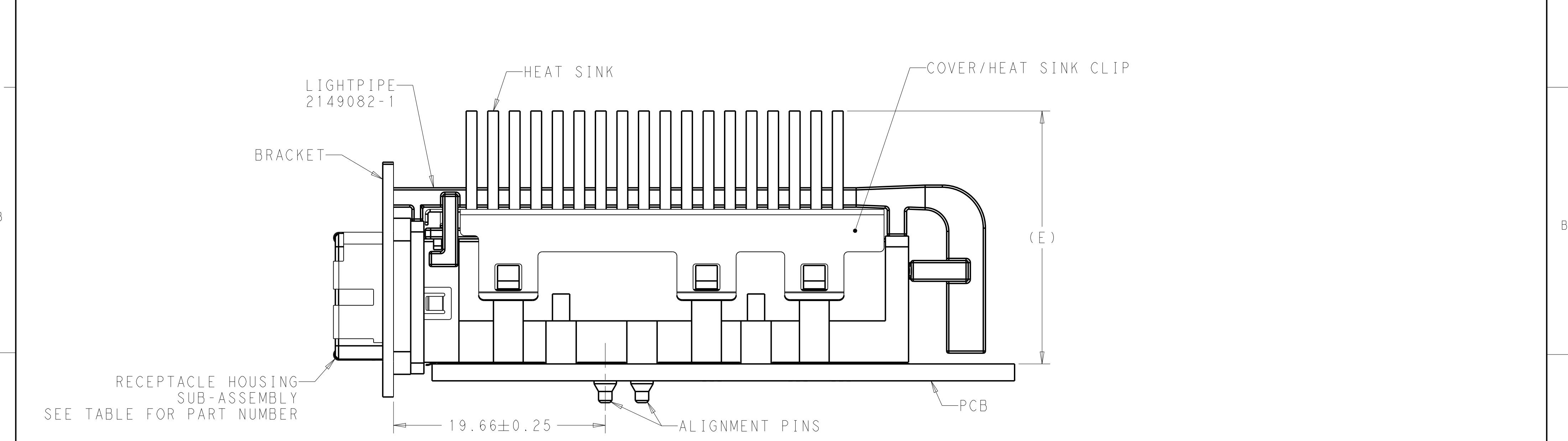
RECOMMENDED BRACKET LOCATION AND HEIGHT OF HEAT SINK MEASURED FROM PCB SCALE 4:1
