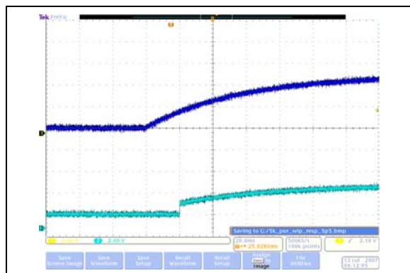
FIGURE 2-14: 5 k \Omega – Power-Up Wiper Response Time (20 ms/Div).
