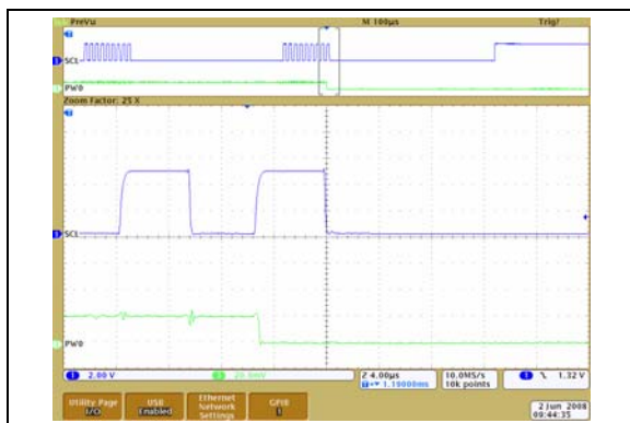
FIGURE 2-45: 100 kΩ – Low-Voltage Decrement Wiper Settling Time ( V_{DD} = 5.5\text{V} ) (1 μs/Div).
