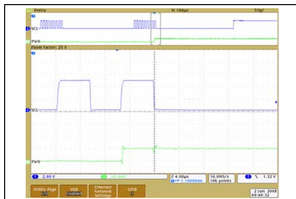
FIGURE 2-47: 100 kΩ – Low-Voltage Increment Wiper Settling Time ( V_{DD} = 5.5\text{V} ) (1 μs/Div).
