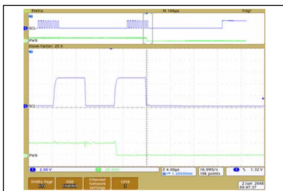
FIGURE 2-46: 100 kΩ – Low-Voltage Decrement Wiper Settling Time ( V_{DD} = 2.7\text{V} ) (1 μs/Div).
