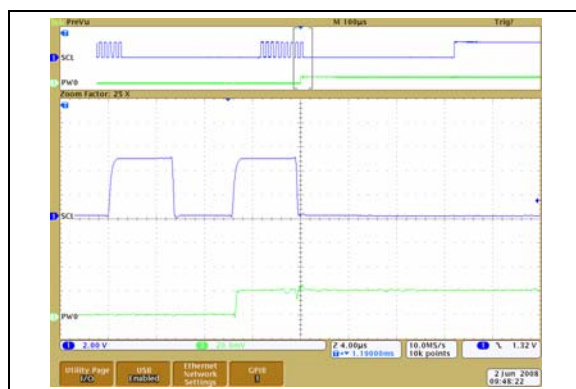
FIGURE 2-48: 100 kΩ – Low-Voltage Increment Wiper Settling Time ( V_{DD} = 2.7\text{V} ) (1 μs/Div).
