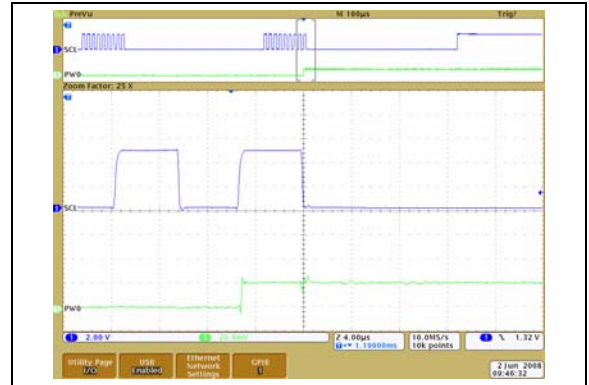
FIGURE 2-47: 100 k \Omega – Low-Voltage Increment Wiper Settling Time ( V_{DD} = 5.5\text{V} ) (1 \mu\text{s}/\text{Div} ).
