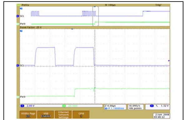
FIGURE 2-48: 100 k \Omega – Low-Voltage Increment Wiper Settling Time ( V_{DD} = 2.7\text{V} ) (1 \mu\text{s}/\text{Div} ).
