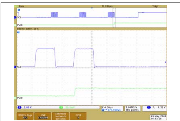
FIGURE 2-38: 50 k \Omega – Low-Voltage Increment Wiper Settling Time ( V_{DD} = 2.7V ) (1 \mu s/Div ).
