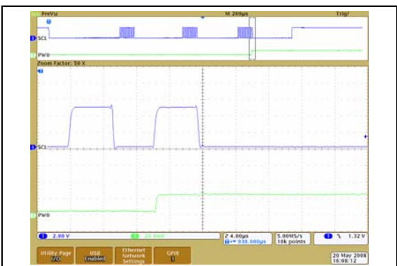
FIGURE 2-37: 50 k \Omega – Low-Voltage Increment Wiper Settling Time ( V_{DD} = 5.5V ) (1 \mu s/Div ).
