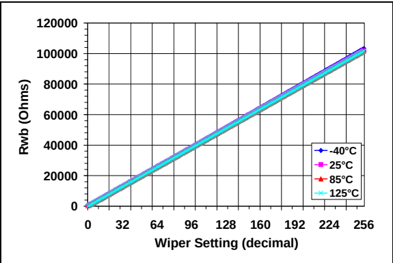
FIGURE 2-44: 100 k\Omega – R_{WB} ( \Omega ) vs. Wiper Setting and Ambient Temperature.
