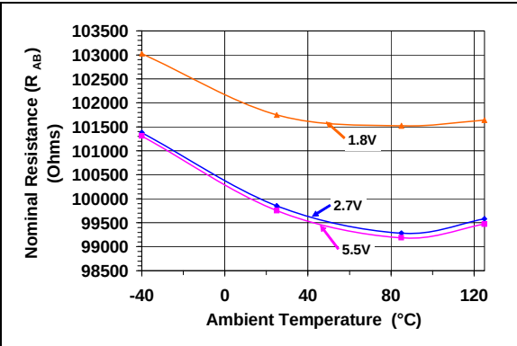
FIGURE 2-43: 100 k\Omega – Nominal Resistance ( \Omega ) vs. Ambient Temperature and V_{DD} .
