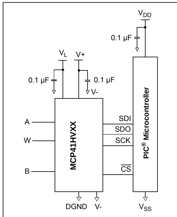
FIGURE 8-11: Typical Microcontroller Connections.
