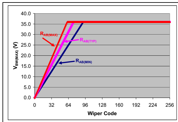
FIGURE 5-7: Maximum V_{BW} vs Wiper Code (5 k \Omega and 10 k \Omega devices).
