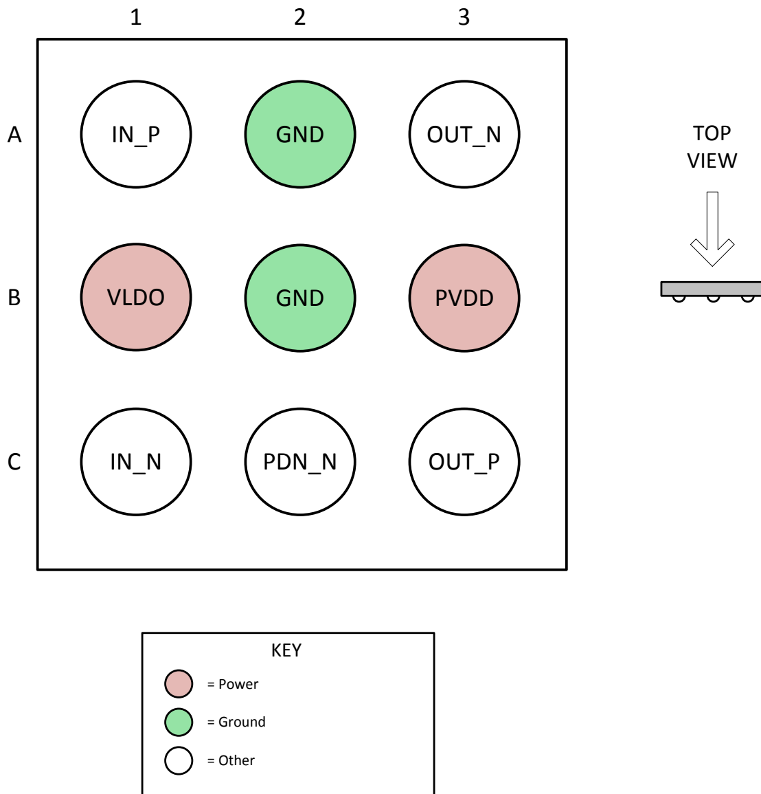
Figure 2: Connection diagram
