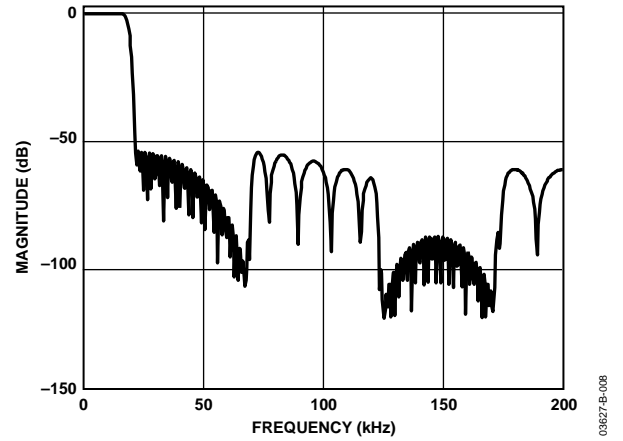
Figure 8. DAC Composite Filter Response, f_s = 48 kHz
