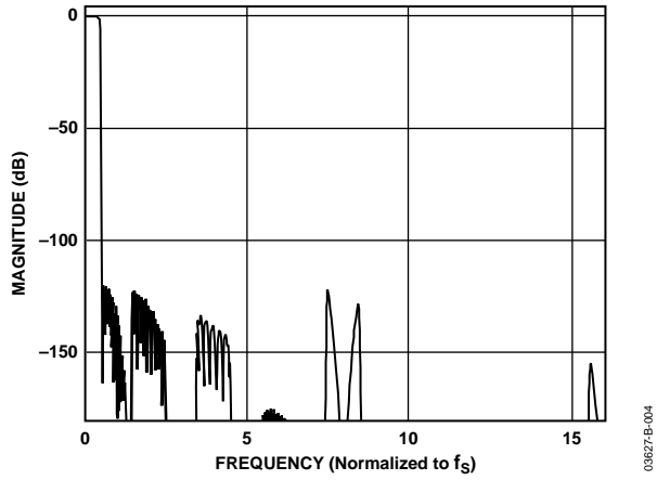
Figure 4. ADC Composite Filter Response
