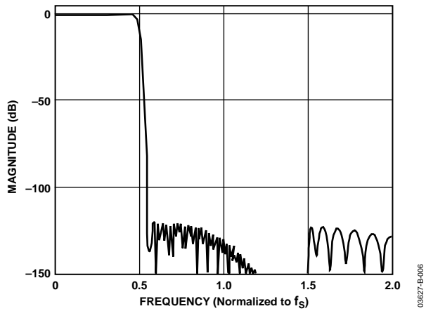
Figure 6. ADC Composite Filter Response (Pass-Band Section)
