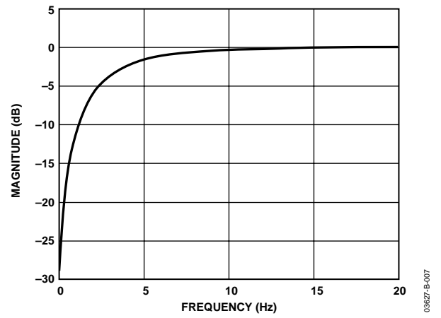
Figure 7. ADC High-Pass Filter Response, f_s = 96 kHz
