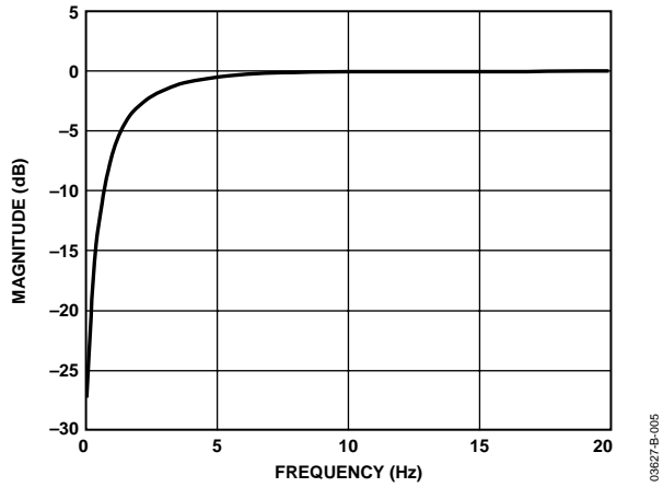
Figure 5. ADC High-Pass Filter Response, f_s = 48 kHz
