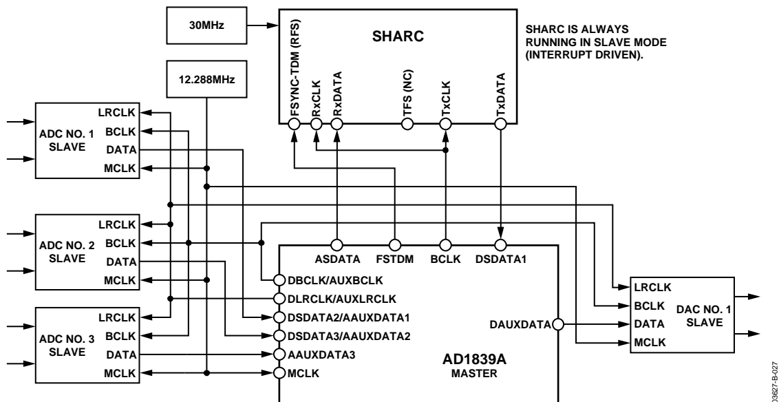
Figure 26. Auxiliary Mode Connection (Master Mode) to SHARC
