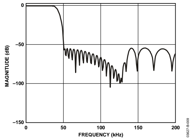
Figure 9. DAC Composite Filter Response, f_s = 96 kHz
