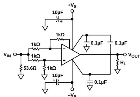
Figure 45. Common-Mode Rejection
