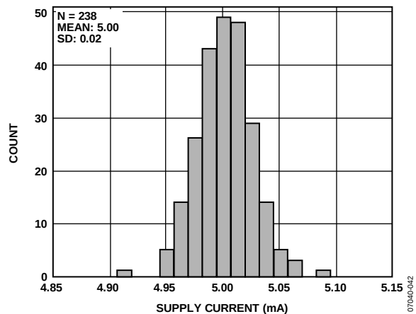
Figure 39. Supply Current
