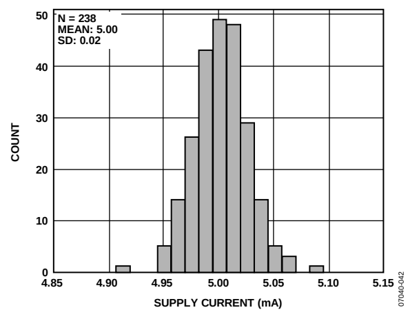
Figure 39. Supply Current
