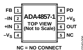
Figure 6. 8-Lead SOIC Pin Configuration
