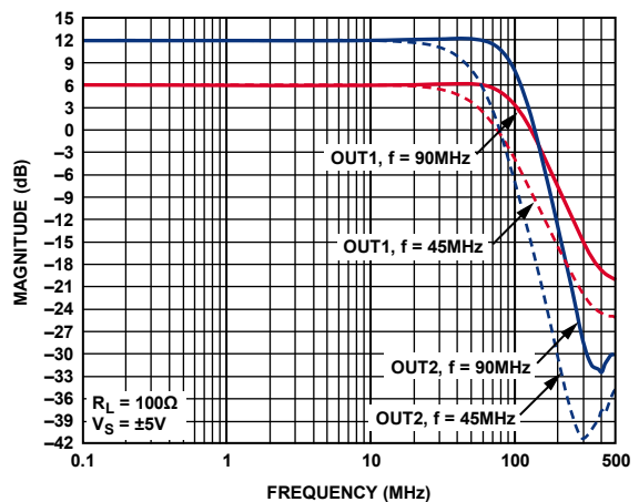
Figure 48. Low-Pass Filter Response
