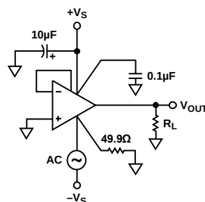
Figure 46. Negative Power Supply Rejection
