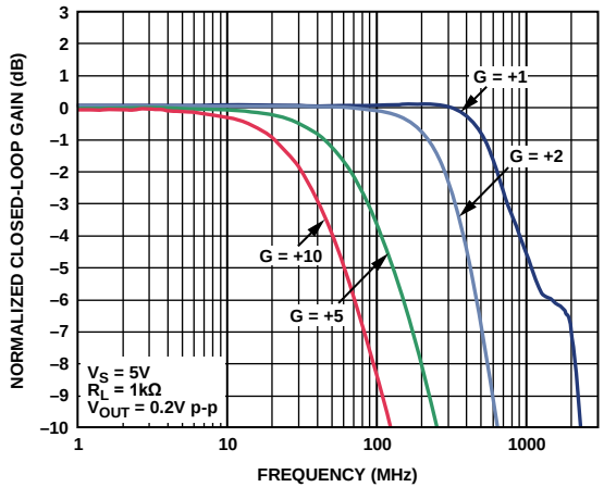
Figure 15. Small Signal Frequency Response for Various Gains (LFCSP)
