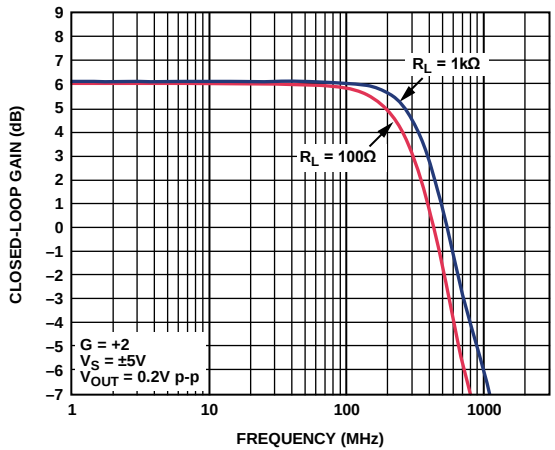
Figure 14. Small Signal Frequency Response for Various Resistive Loads (LFCSP)
