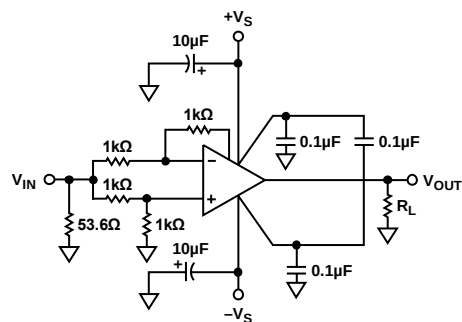
Figure 45. Common-Mode Rejection
