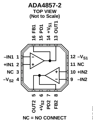
Figure 3. 16-Lead LFCSP (CP)
