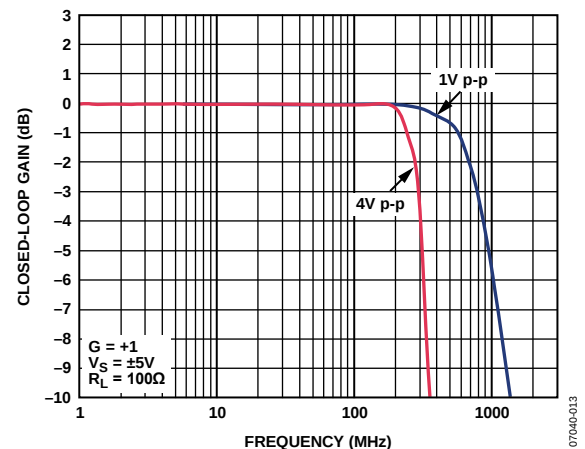
Figure 13. Large Signal Frequency Response vs. V_{OUT} (LFCSF)
