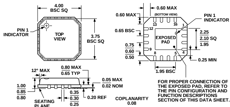
Figure 53. 16-Lead Lead Frame Chip Scale Package [LFCSP_VQ] 4 mm x 4 mm Body, Very Thin Quad (CP-16-4) Dimensions shown in millimeters
