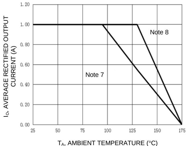
Fig. 5 DC Forward Current Derating
