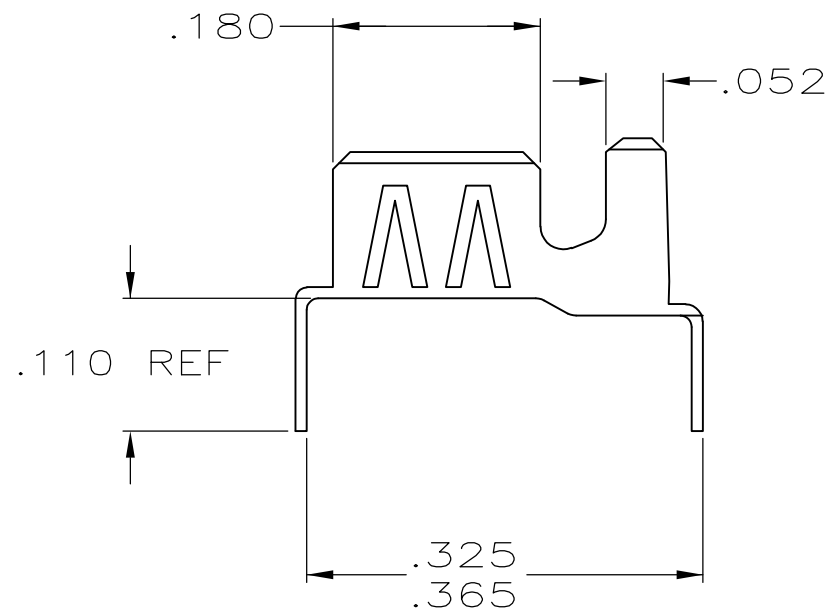
VIEW D
