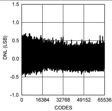
Figure 7. DNL - 250 kSPS
