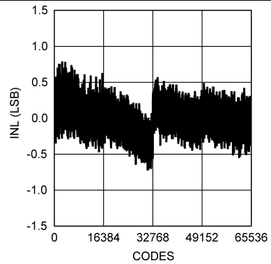
Figure 8. INL - 250 kSPS
