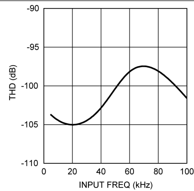
Figure 24. THD vs. INPUT Frequency
