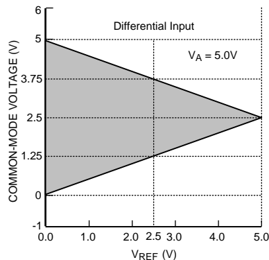
Figure 44. V_{CM} range for Differential Input operation
