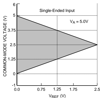
Figure 46. V_{CM} Range for single-Ended Operation
