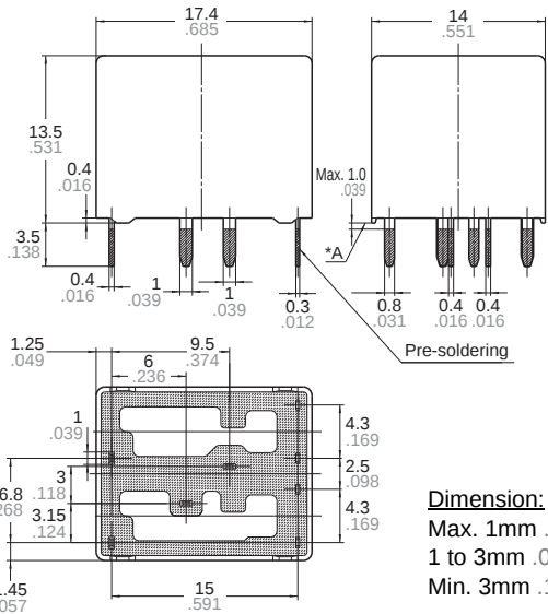
External dimensions
