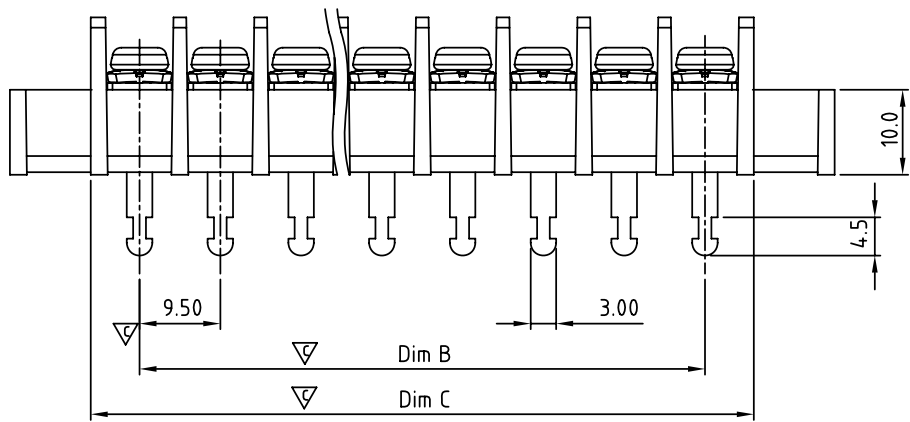
Dimension A&B&C
