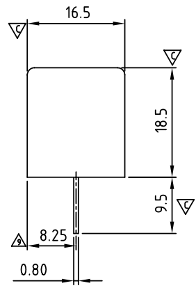
Dimension A&B&C
