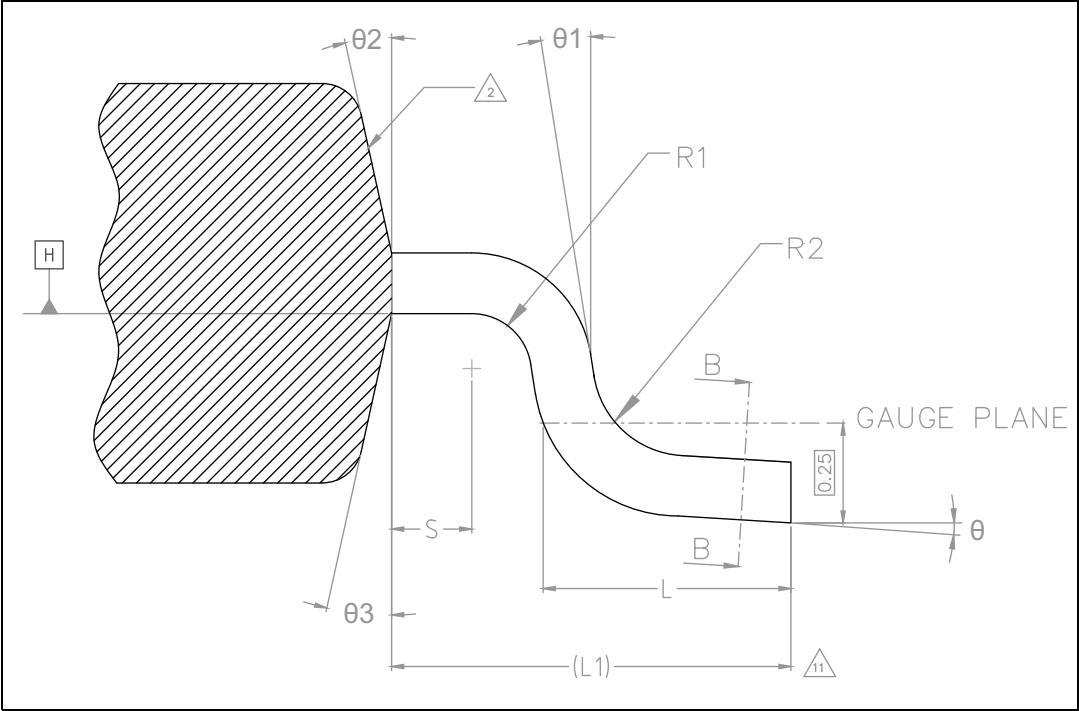
Figure 48. eTQFP100 section A-A
