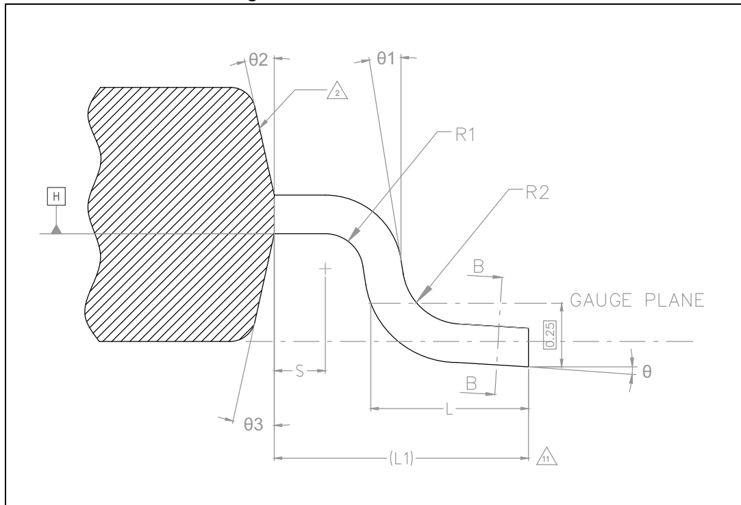
Figure 57. eLQFP176 section B-B
