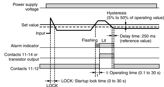
Overcurrent Operation Diagram (Output Drive Method: Normally Open) DIP switch setting: SW3 OFF, SW4 OFF
