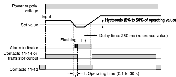
Undercurrent Operation Diagram (Output Drive Method: Normally Closed) DIP switch setting: SW3 ON, SW4 ON
