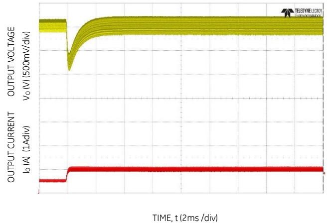
Figure 22. Transient Response to Dynamic Load Change from 0.6 to 1.1A at 12Vin, C out =7x4.7uf, C Tune =82pF, R Tune =40.2kΩ
