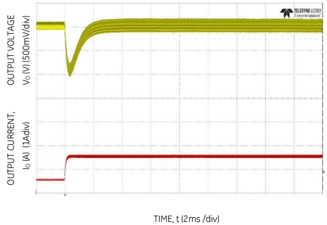
Figure 10. Transient Response to Dynamic Load Change from 0.6 to 1.6A at 12Vin, C_{out}=10 \times 4.7\mu\text{F} , C_{Tune}=560\text{pF} , R_{Tune}=40.2\text{k}
