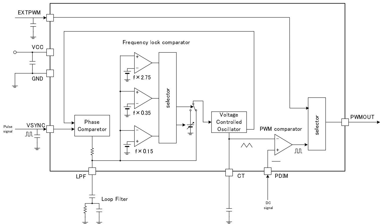
Figure 6. Block Diagram
