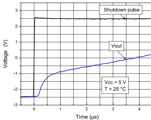
Figure 22: Turn-on time, V_{\text{CC}} = 5 V, Vout pulled down, T = 25^\circ\text{C}
