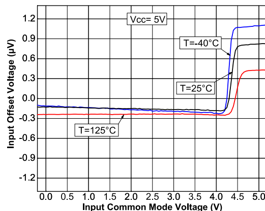
Figure 19: Input offset voltage vs. input common mode at V_{CC} = 5 V
