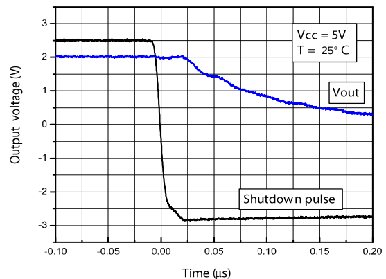
Figure 23: Turn-off time, V_{\text{CC}} = 5 V, Vout pulled down, T = 25^\circ\text{C}
