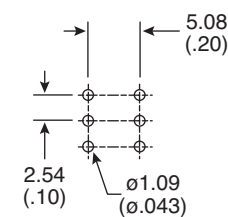
P.C. Mounting
