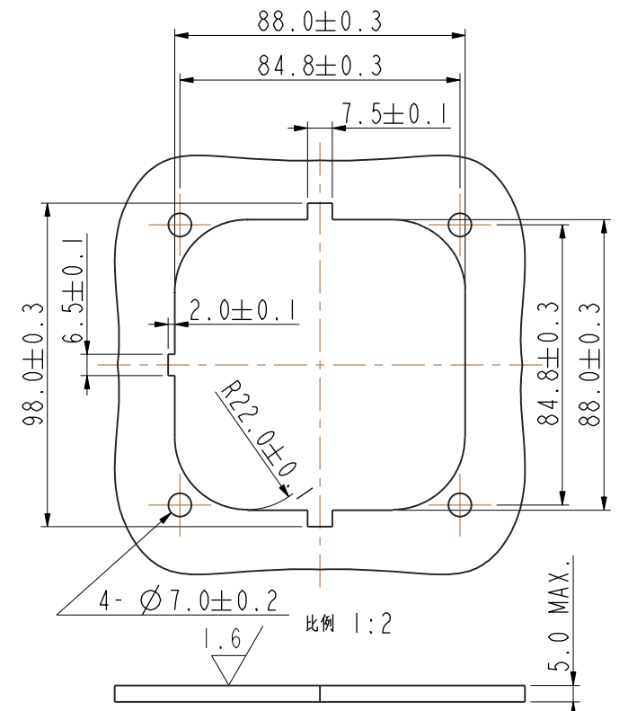
REAR MOUNTING INTERFACE SPECIFICATION 后安装板面参考安装尺寸
