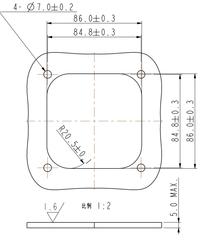
FRONT MOUNTING INTERFACE SPECIFICATION 前安装板面参考安装尺寸
