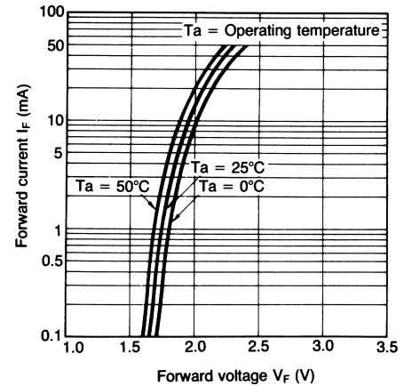
LED Characteristics ( V_F vs. I_F Characteristics) (Green)
