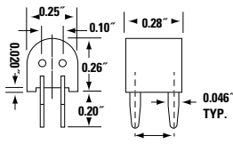
Circuit Board Mounting Detail
