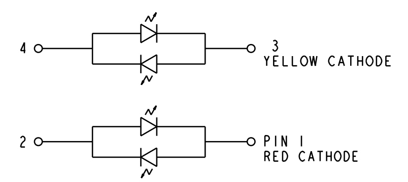
SCHEMATIC FOR CENTER BI-LEVEL
