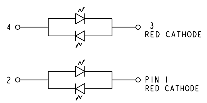
SCHEMATIC FOR LEFT & RIGHT BI-LEVEL
