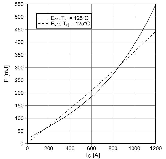
Schaltverluste IGBT-Wechselr. (typisch) switching losses IGBT-inverter (typical) E_{on} = f(I_c) , E_{off} = f(I_c) V_{GE} = \pm 15\text{ V} , R_{Gon} = 2,4\ \Omega , R_{Goff} = 3\ \Omega , V_{CE} = 900\text{ V}
