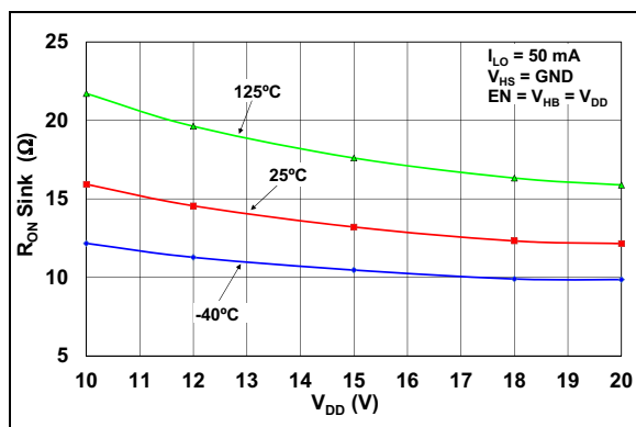
FIGURE 2-13: LO Output Sink ON-Resistance vs. V_{DD} .
