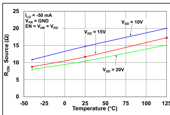
FIGURE 2-18: LO Output Source ON-Resistance vs. Temperature.
