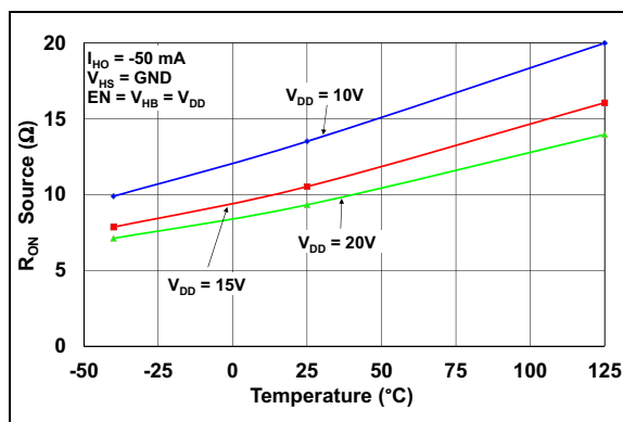
FIGURE 2-16: HO Output Source ON-Resistance vs. Temperature.
