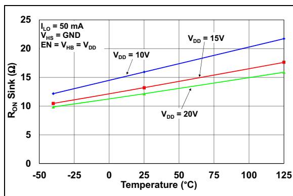
FIGURE 2-14: LO Output Sink ON-Resistance vs. Temperature.
