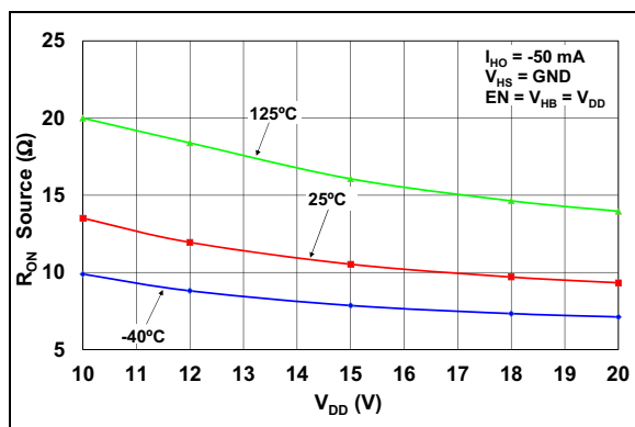
FIGURE 2-15: HO Output Source ON-Resistance vs. V_{DD} .
