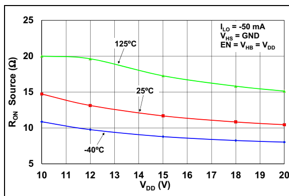
FIGURE 2-17: LO Output Source ON-Resistance vs. V_{DD} .
