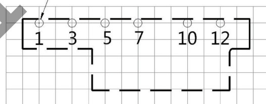
Top View PCB Layout
