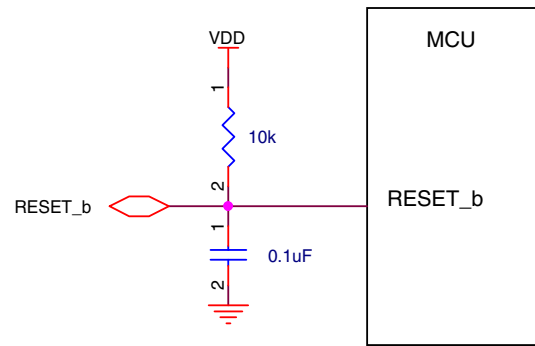
Figure 30. Reset circuit
