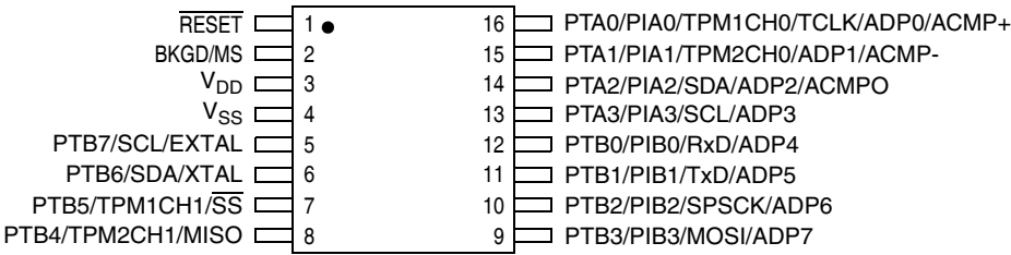
Figure 2-2. 16-Pin TSSOP
