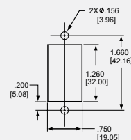
Mounting Detail Single, Two & Three Pole
