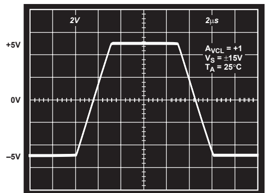
Figure 27. Large Signal Transient Response
