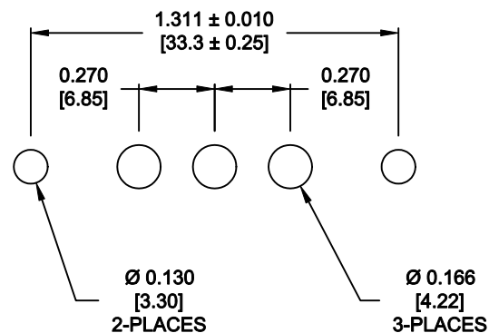
RECOMMENDED PCB LAYOUT TOLERANCE \pm 0.002 [0.05]
